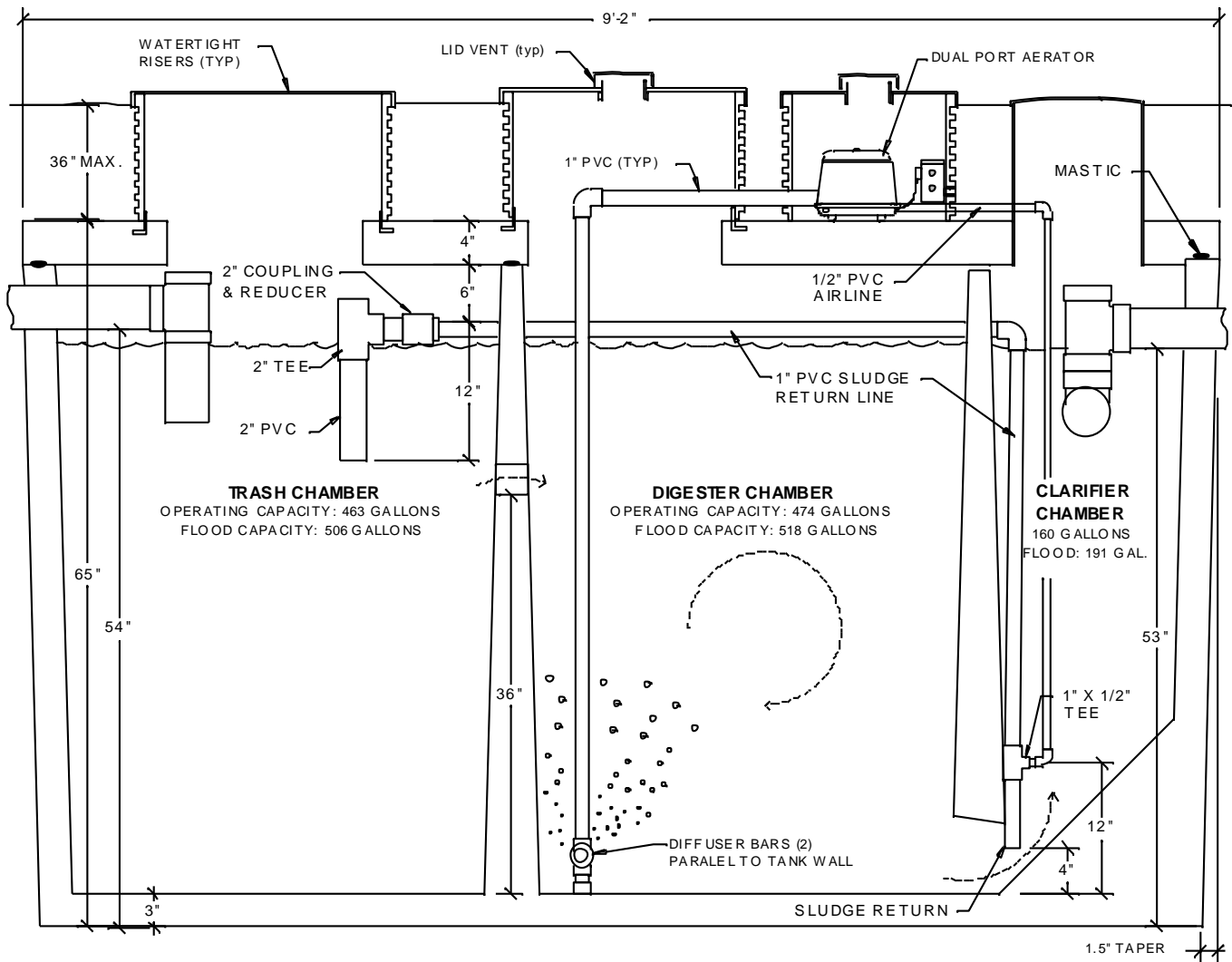
SIDE VIEW
